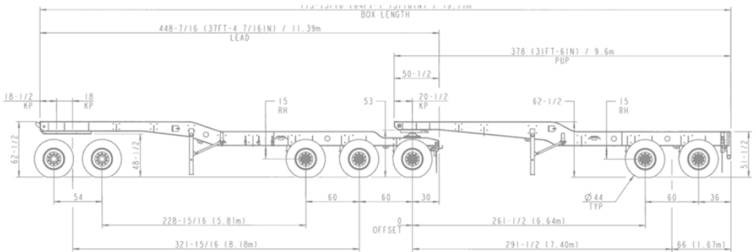
MAIN B-TRAIN TRAILER LAYOUT
